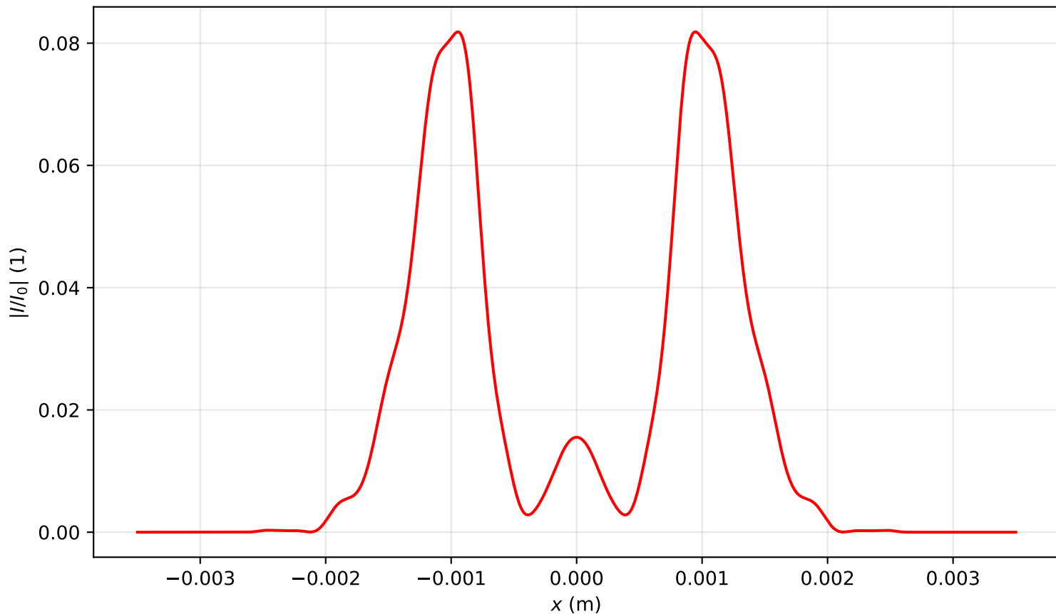
Intensity profile I(x, y = 0, z = 3.105)/I_0 , P_{in}=7.5P_{cr} , artificial time
